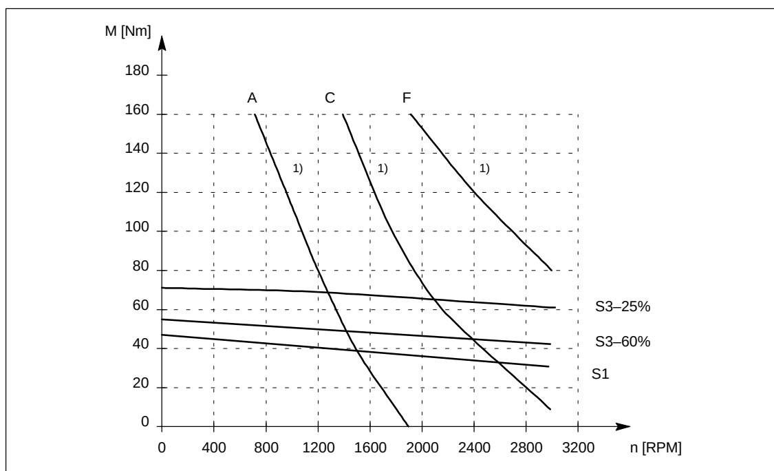
Fig. 3-13 Speed–torque diagram 1FT5104
