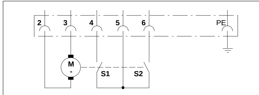
Fig. 1-7 Circuit diagram
