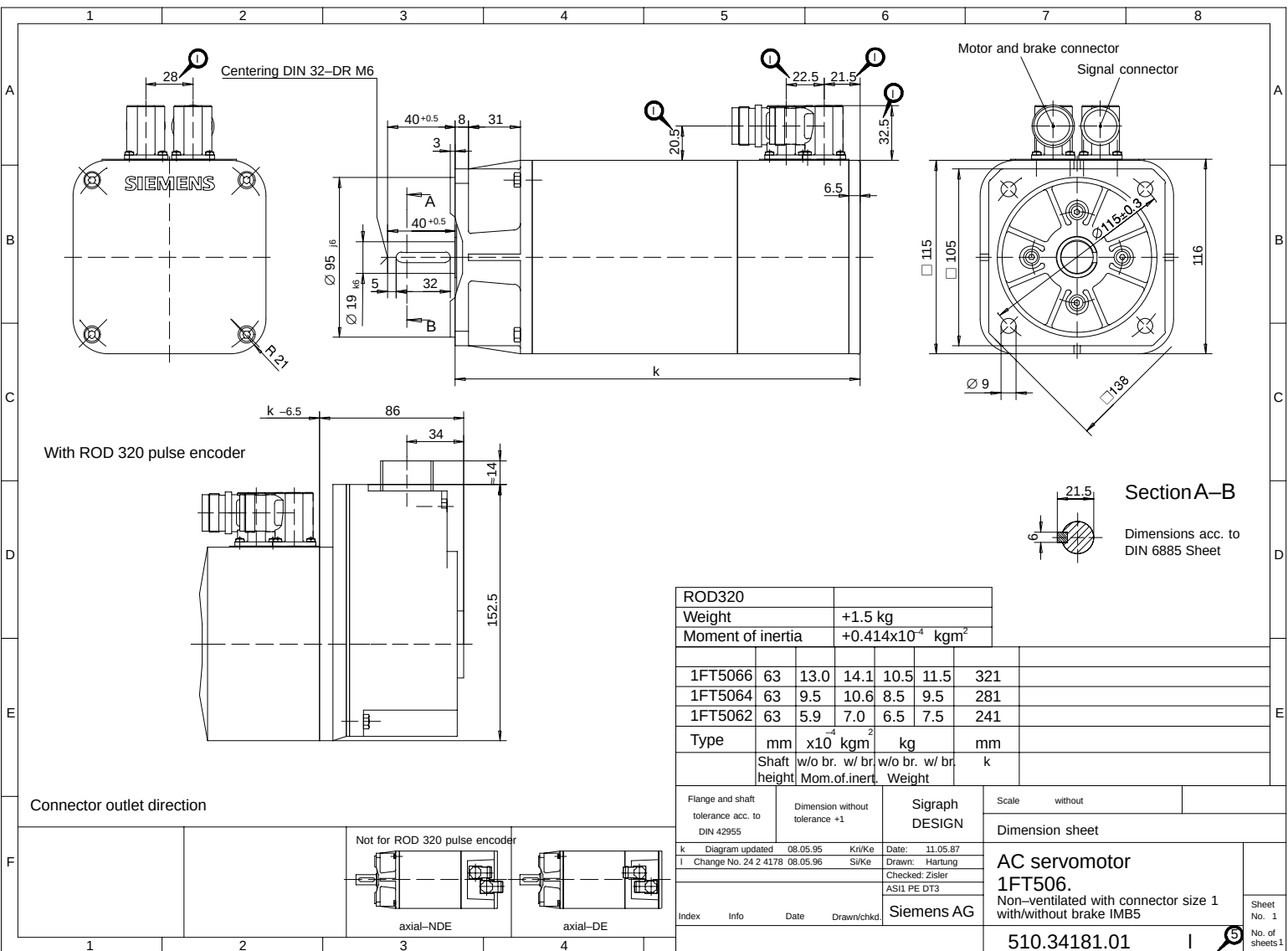
Fig. 4-3 1FT506 □ non-ventilated with connector size 1
