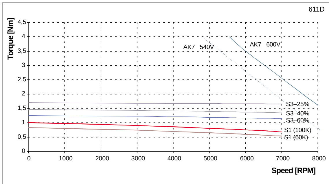
Fig. 3-3 Speed–torque diagram 1FT6031
