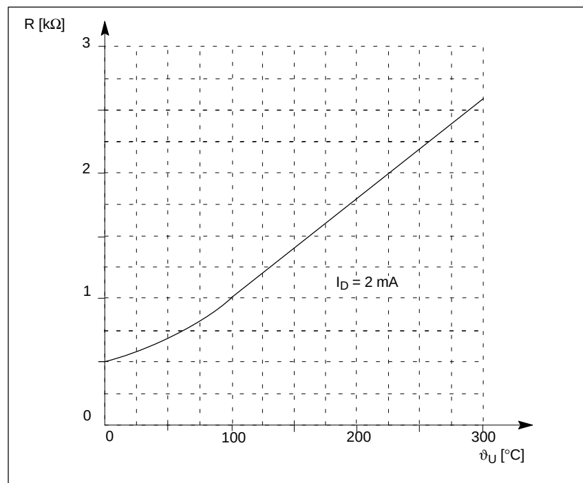
Fig. 1-7 Temperature characteristic
