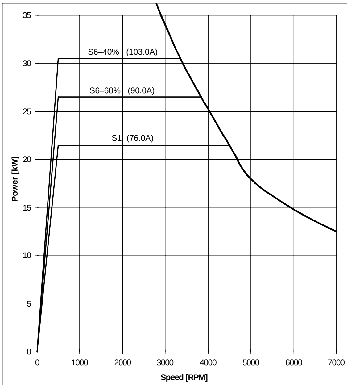
Fig. 3-49 Speed–power diagram 1PH7184–□NT□□
