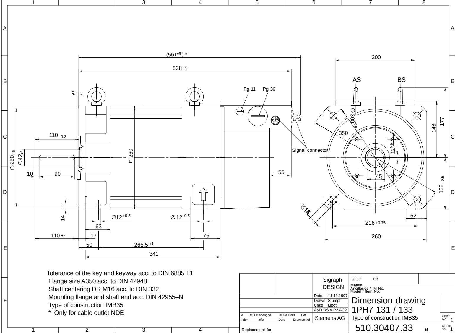
Fig. 4-8 1PH7 131/133, type of construction IM B35
