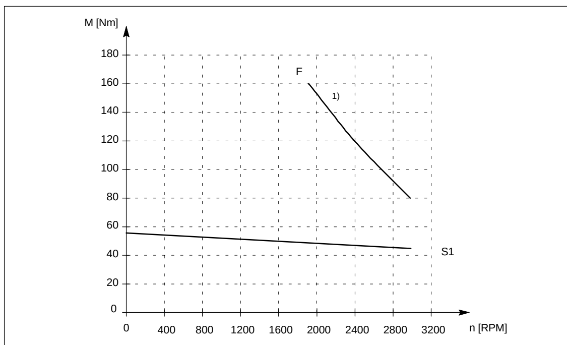
Fig. 3-23 Speed–torque diagram 1FT5104. force–ventilated
