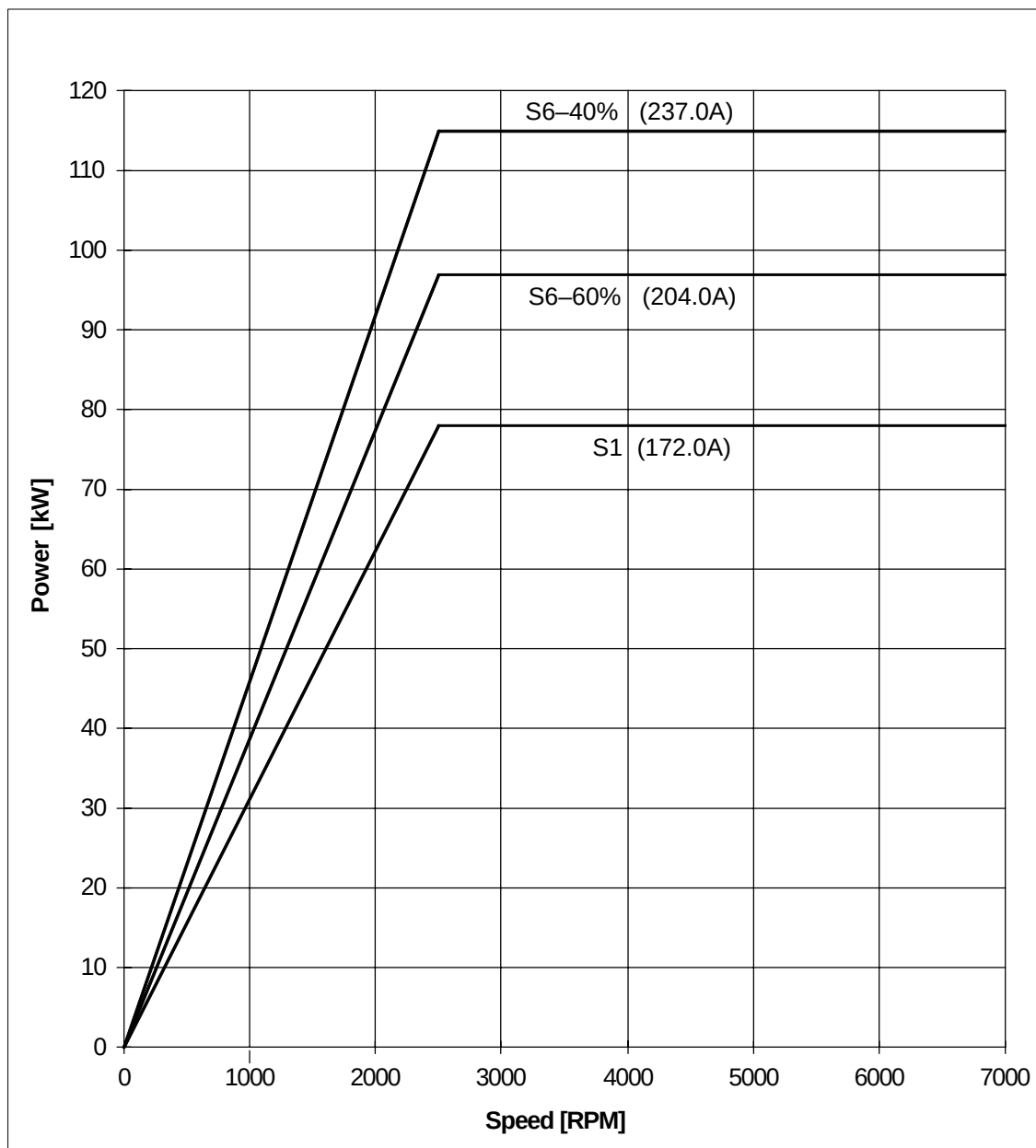
Fig. 3-53 Speed–power diagram 1PH7184–□NL□□
