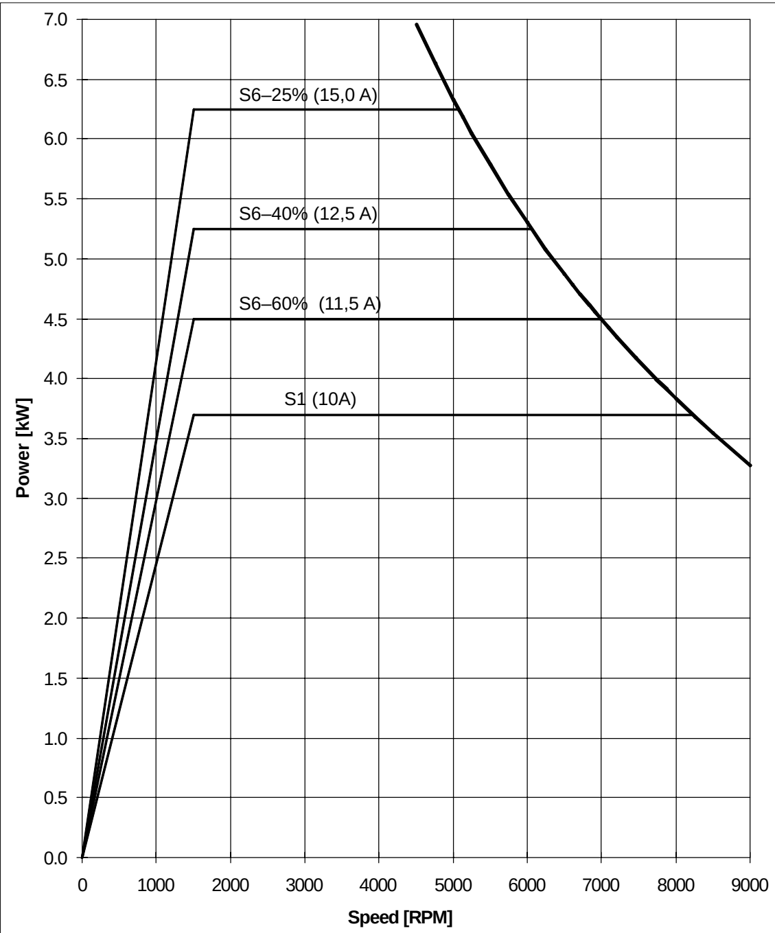
Fig. 3-1 Speed–power diagram 1PH7101–2NF□□
