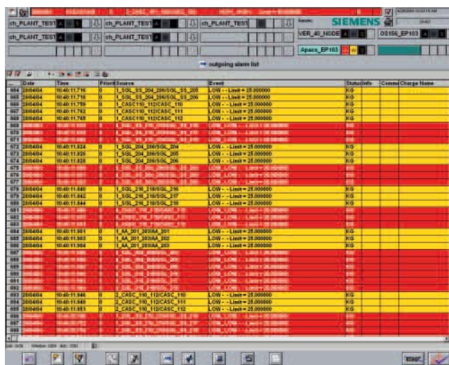
Message window on the operator station
