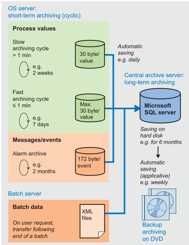
Overview of short-term and long-term archiving
