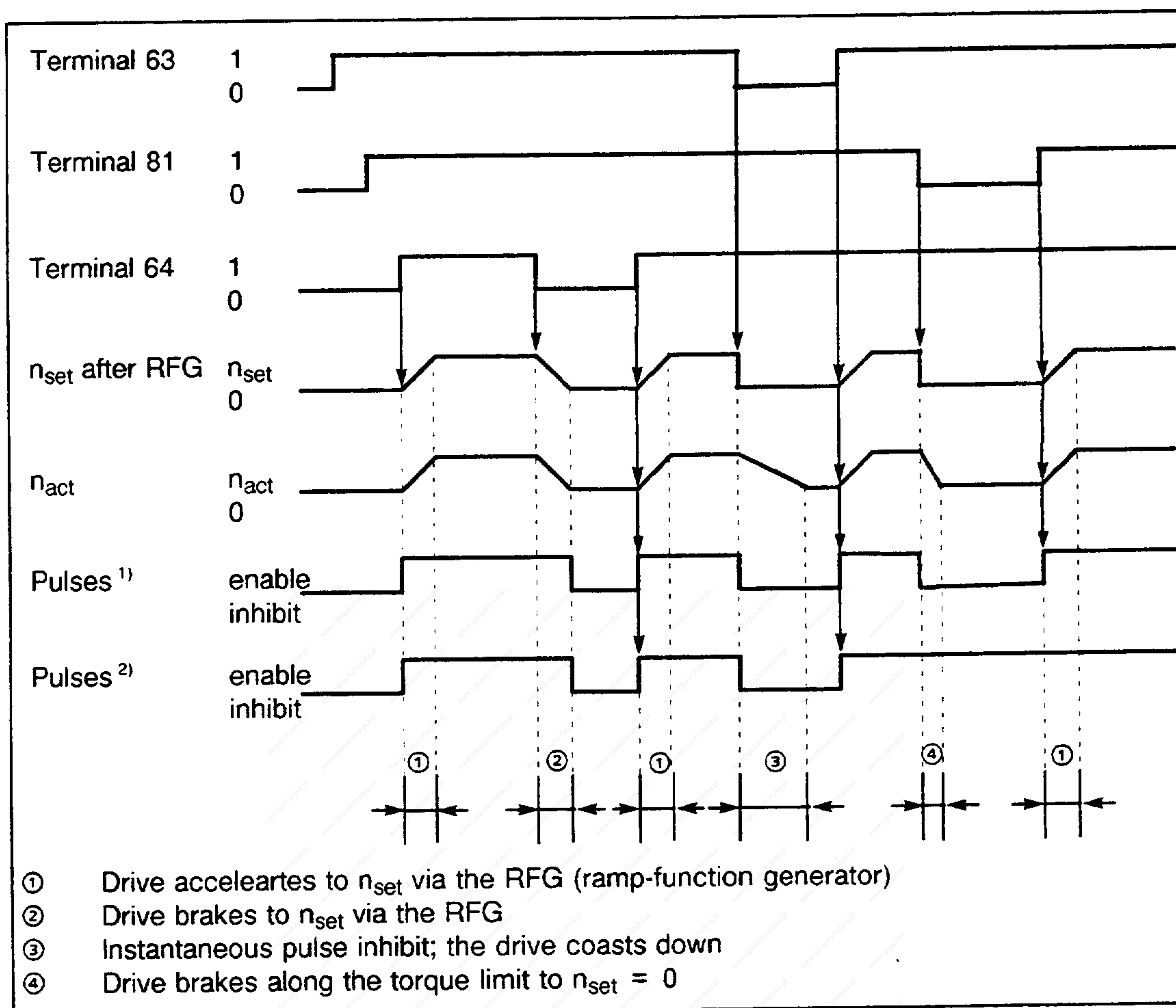
Enable signals
