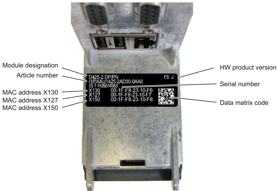
Figure 2-6 MAC addresses of SIMOTION D425-2 DP/PN
