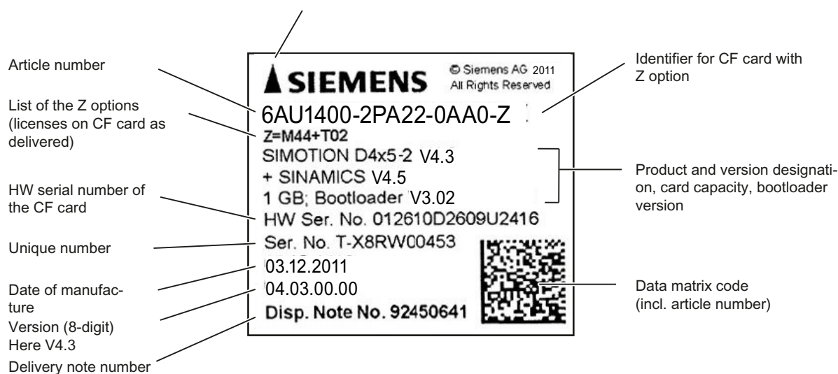
Figure 2-8 Rating plate of the CF card (example of 1 GB CF card)
