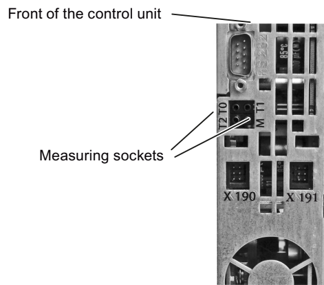
Figure 4-10 Measuring socket position
