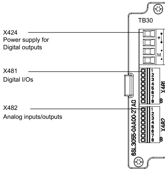
Figure 7-3 Interface arrangement on the TB30
