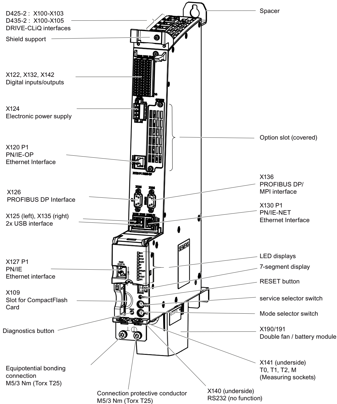
Figure 2-2 D425-2 DP and D435-2 DP representation
