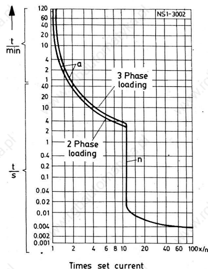
Time current characteristics of 3VU13
