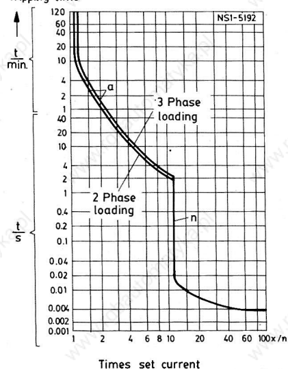
Time current characteristics of 3VU16
