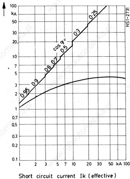
Cut off characteristics of 3VU1300-0MK00
