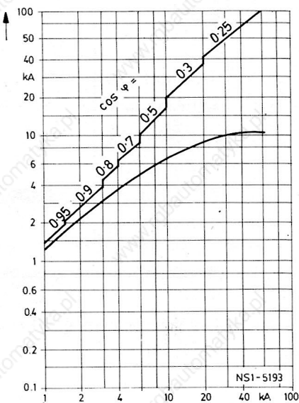
Short circuit current Ik (effective)
