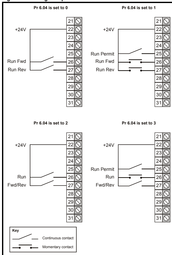
Figure 11-21 Digital input connections when Pr 6.04 is set to 0 to 3
