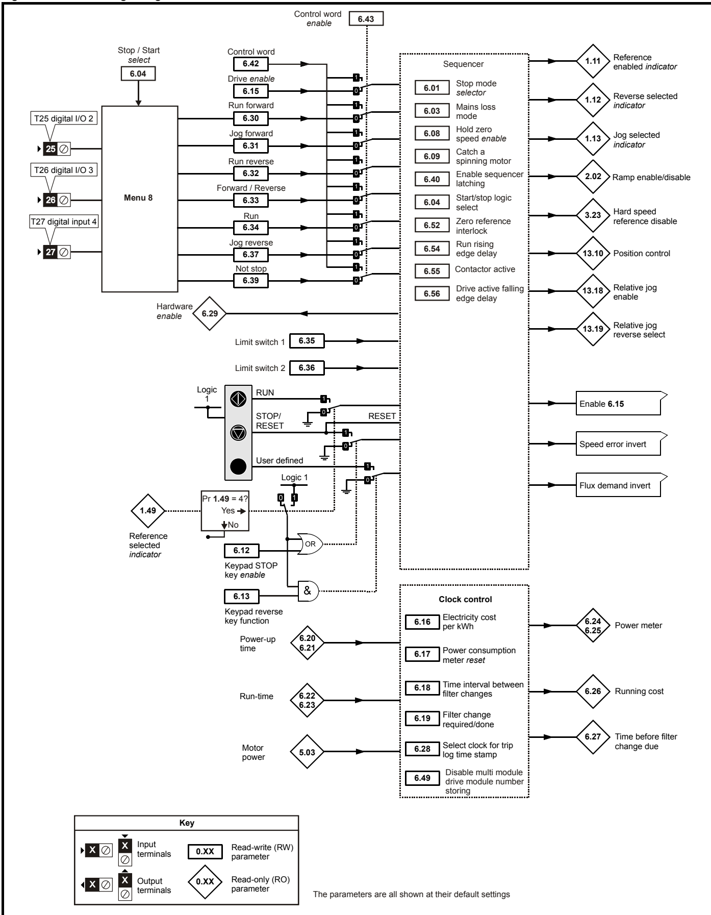
Figure 11-7 Menu 6 logic diagram
