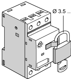
Figure 9-3 Securing the toggle switch (3RV1.1)
