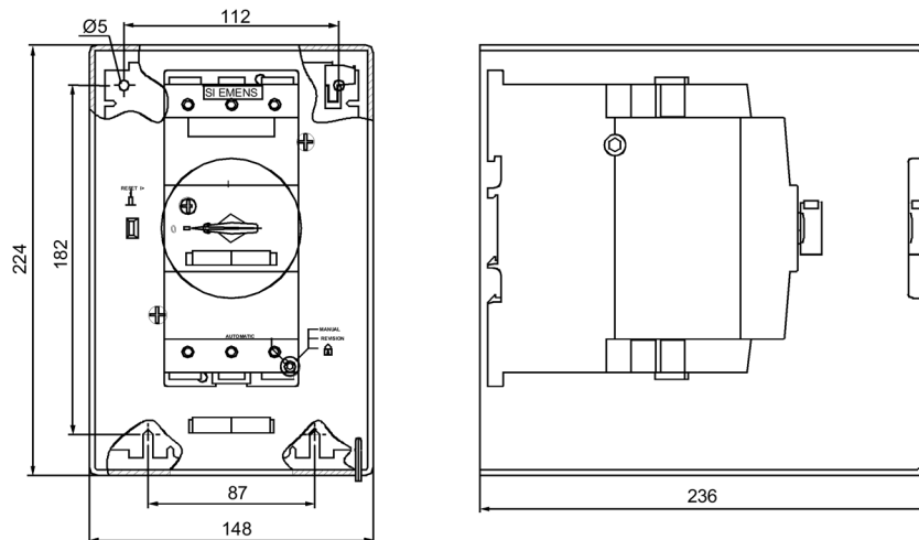
Figure C-44 3RV1946-3A remote motorized operating mechanism
