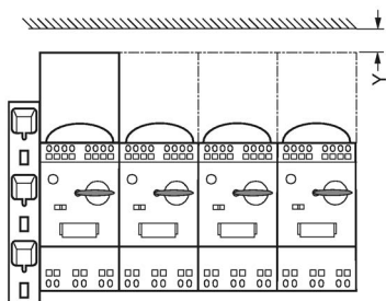
Figure 10-7 Installation guidelines
