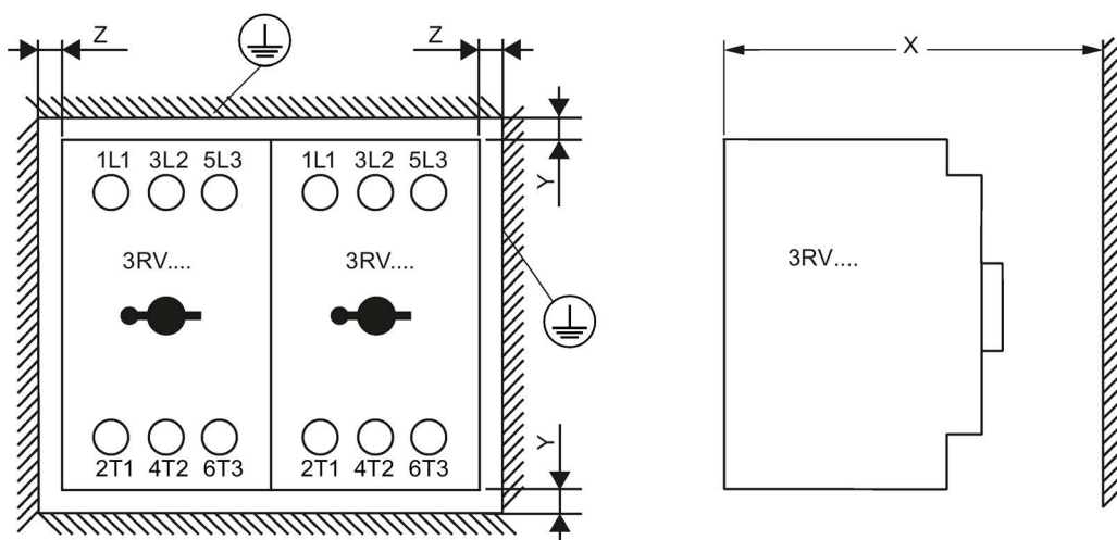
Figure 7-1 Clearances from grounded or live parts
