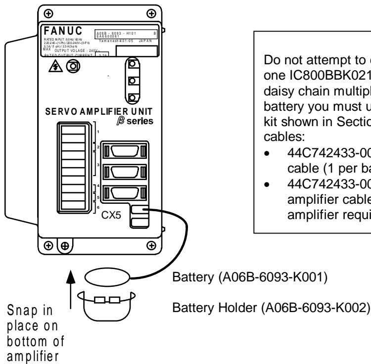
Figure 29. Connecting a single β Series amplifier to an absolute encoder battery pack
