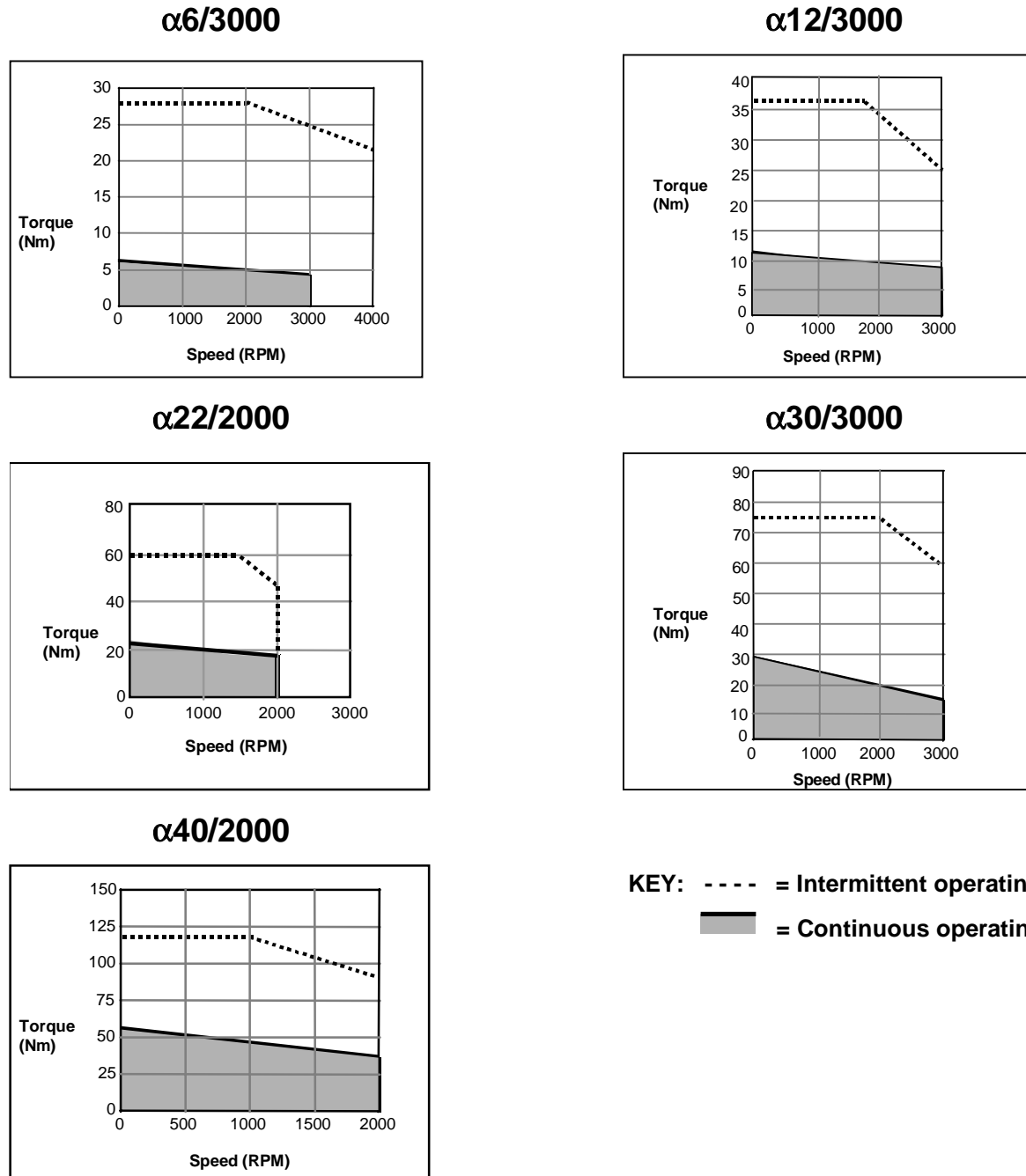
Figure 2. \alpha Series motor speed-torque curves
