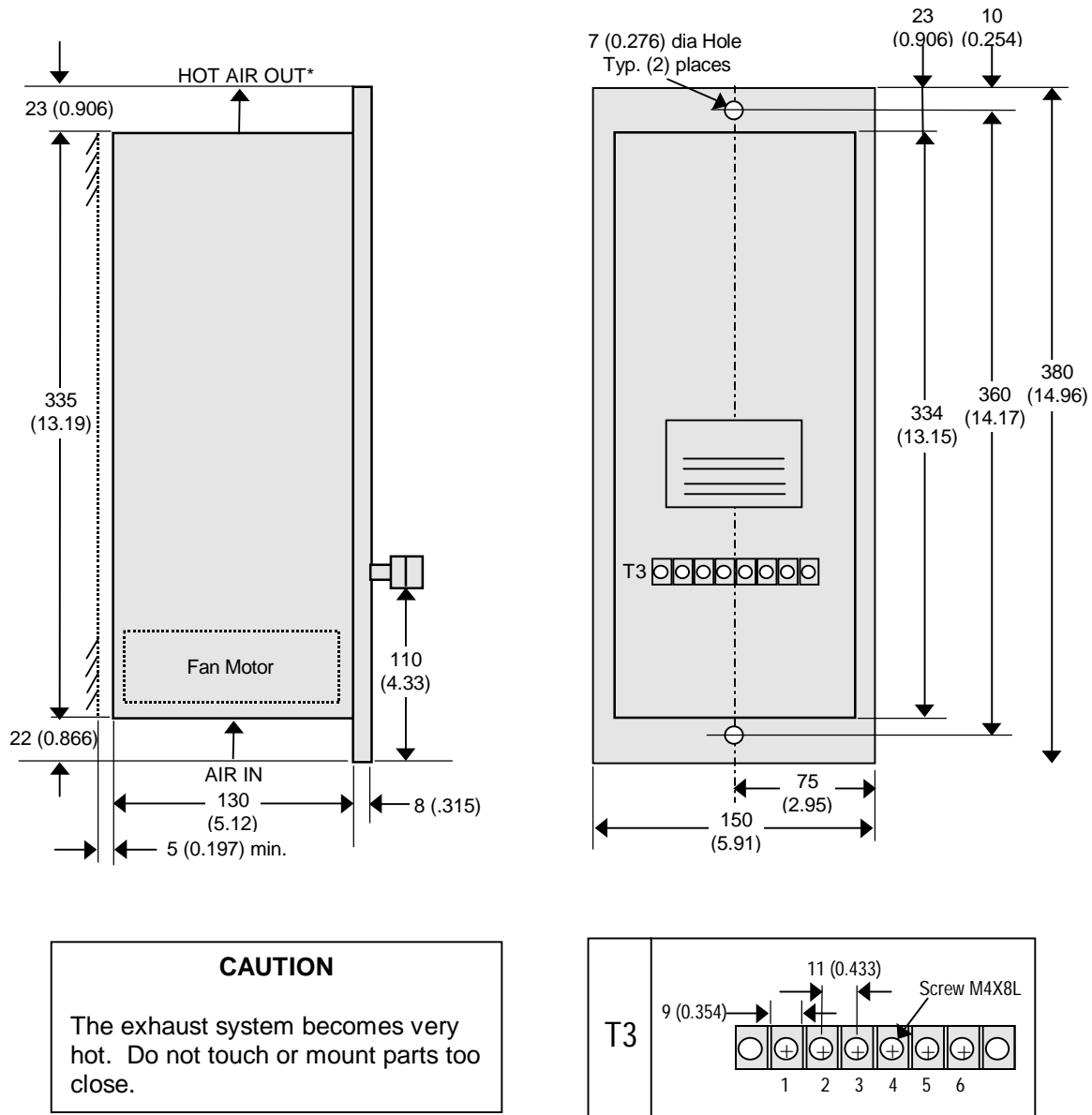
A06B-6089-H711 (800 W) for the α SVU1-130 and A06B-6089-H713 (800W) for the α SVU1-80
